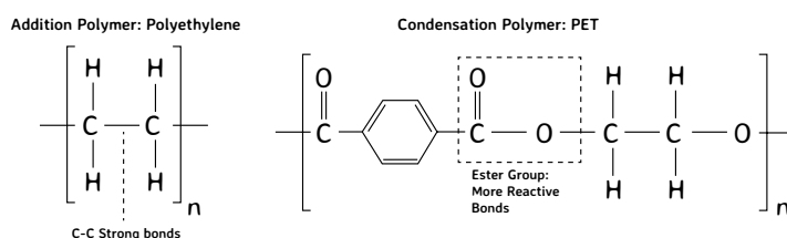
Figure 55: two polymers following different polymerisation routes 44 .
