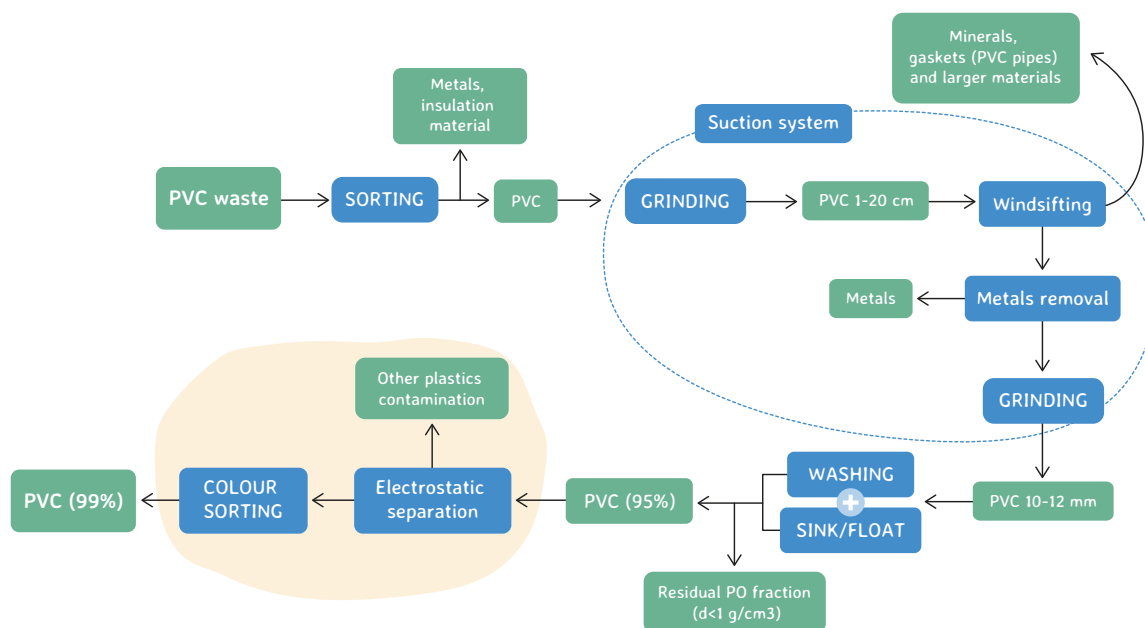
Figure 43. Exemplary flowchart of a PVC recycling line.
