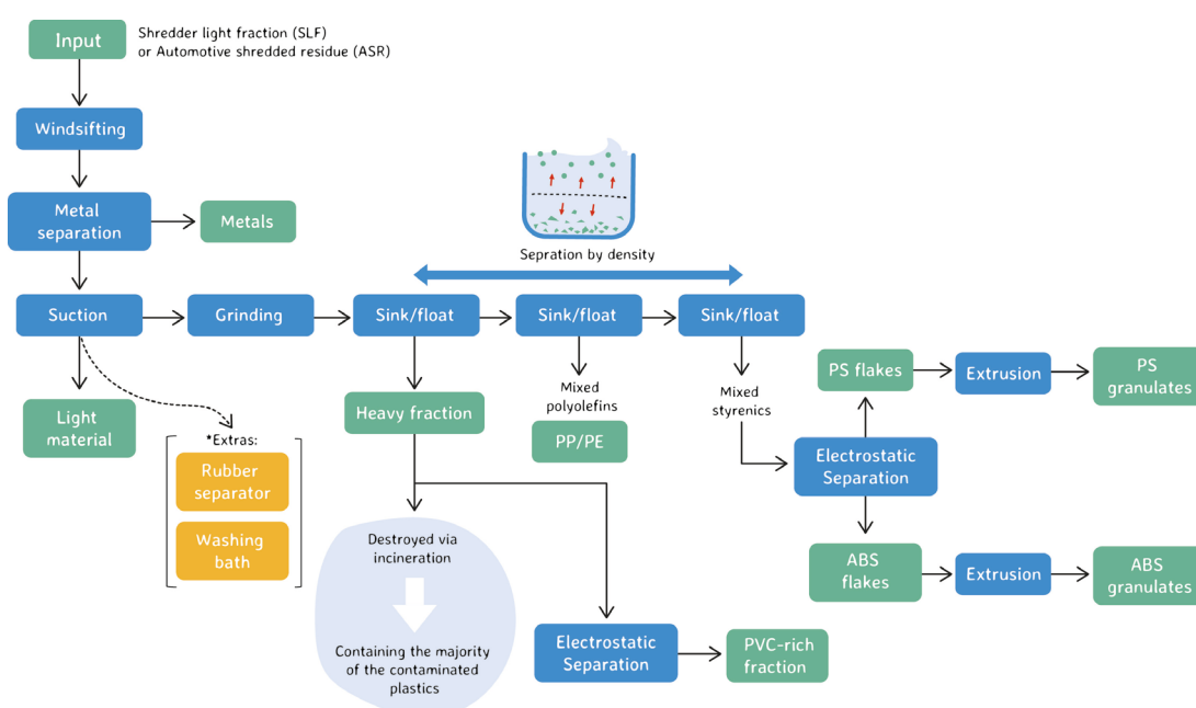
Figure 39. Schematic representation of a recycling process for WEEE and ELV materials. *Post consumer cable sheathing waste is in some cases separated to recover flexible PVC and copper.
